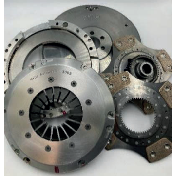
TWIN PLATE SPRUNG PADDLE INTERPLATE & COVER ASSEMBLY Series Part No 80-0000
